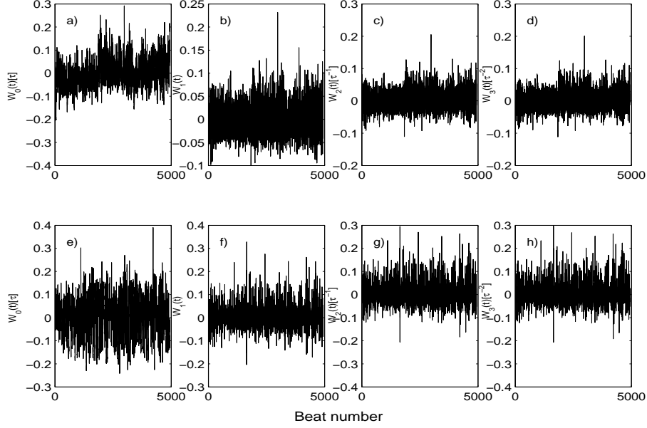
Figure 1: The time series of the first four dynamic orthogonal variables W_i , where i = 0, \dots, 3 for the young (a-d) and the elderly persons (e-h). The time series of the elderly person is accompanied by more significant fluctuations of an R-R interval. The time series of elderly person is characterized by greater frequency of occurrence of significant fluctuations. It shows higher degree of Markovity of the fluctuations of an R-R interval for the elderly person.
